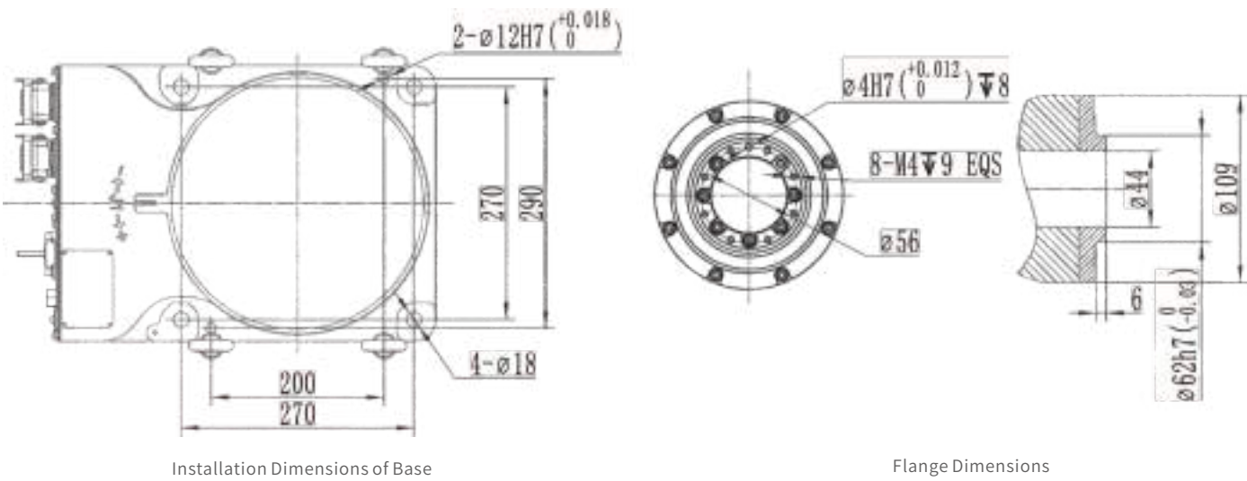
Flange Dimensions
